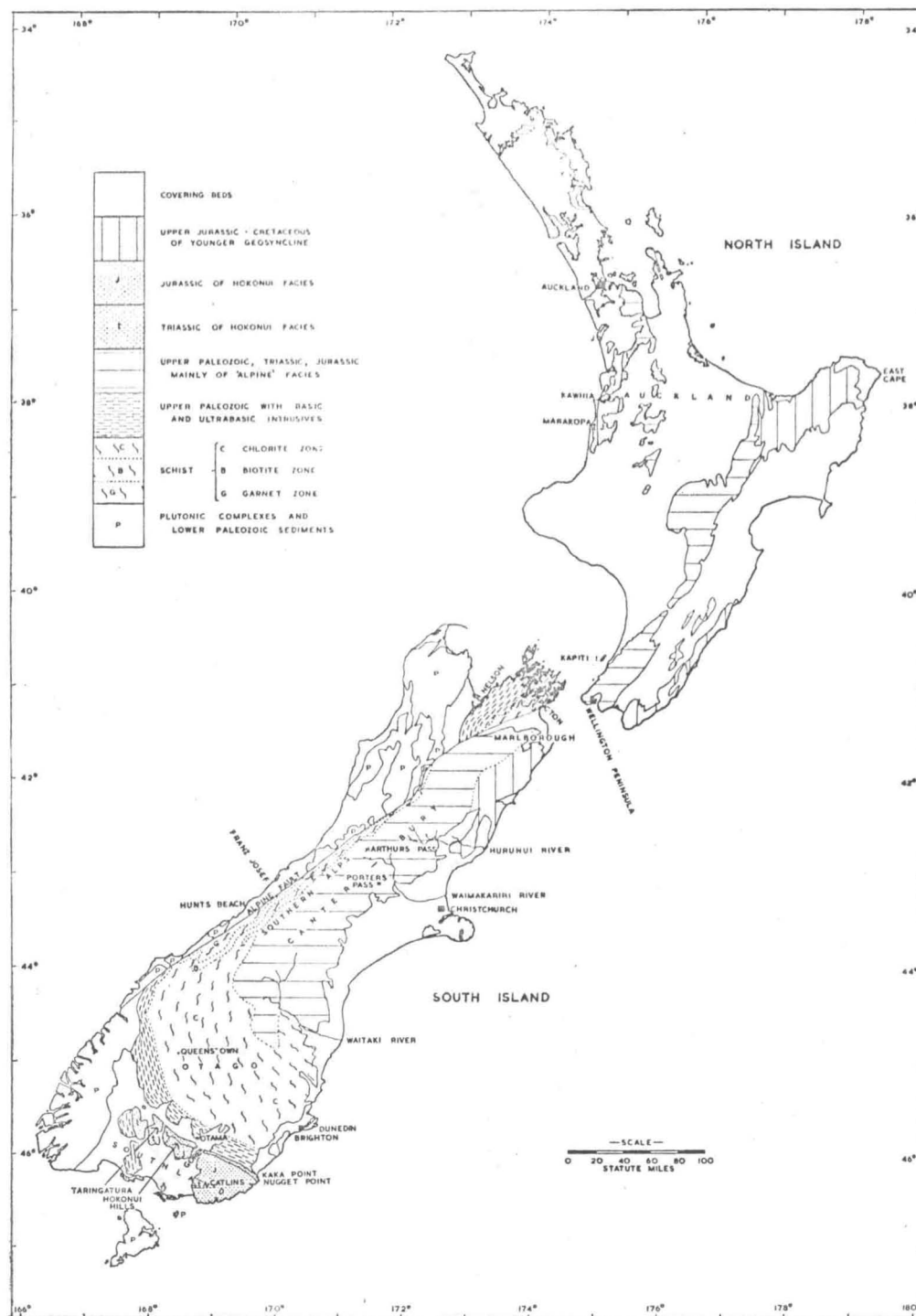
Fig. 1. Geological sketch map showing rocks of the New Zealand Geosyncline (Based on WELLMAN, 1956, and on the 1 : 2,000,000 geological map of New Zealand, N.Z. Geological Survey, 1958).
